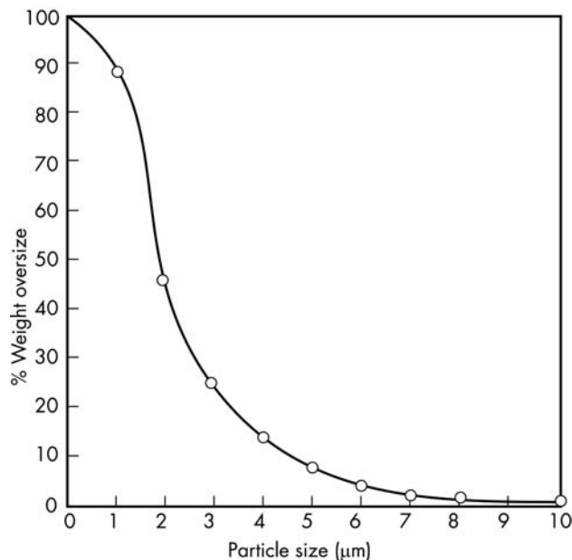
Figure 1: Particle-size distribution of titanium dioxide (fine powder).
