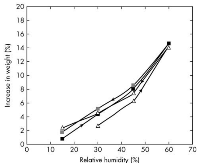
Figure 2: Moisture sorption-desorption isotherm of sulfobutylether \beta -cyclodextrin sodium, at 30°C.
