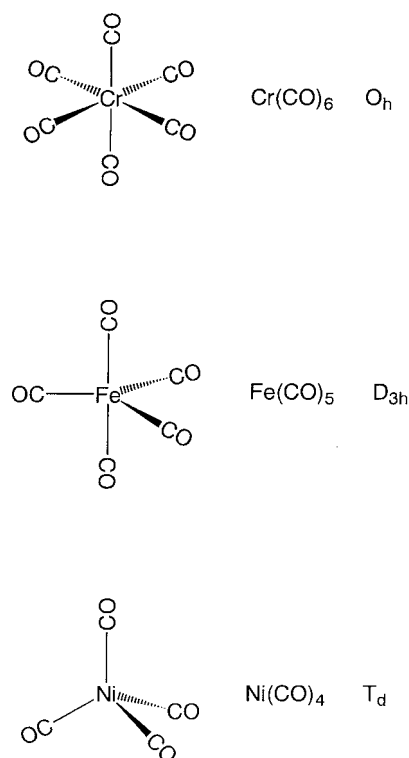
Fig. 6.14 Structures of metal carbonyl compounds.
