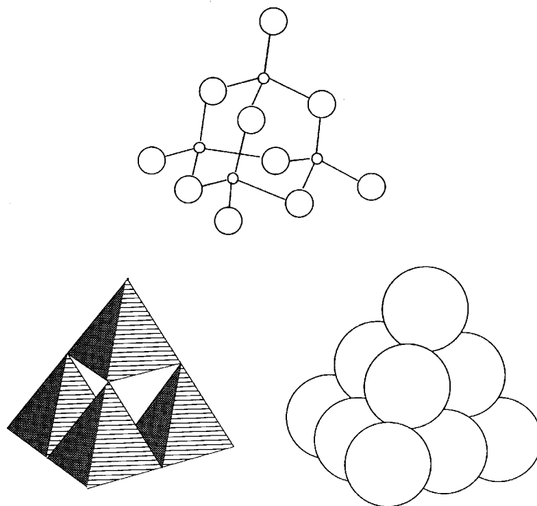
Fig. 2.12 Three expressions for the structure of P_4O_{10} .
