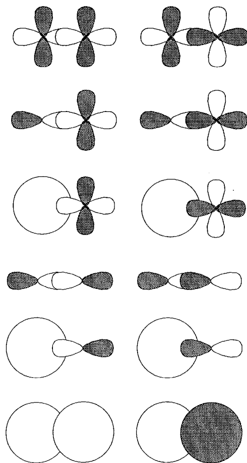
Bonding \sigma orbital Antibonding \sigma^* orbital
