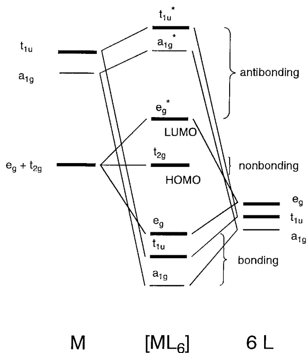
Fig. 6.10 Bonding and anti-bonding M(metal)-L(ligand) molecular orbitals.
