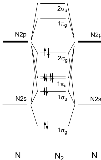
Fig. 2.19 Molecular orbitals of N_2 .
