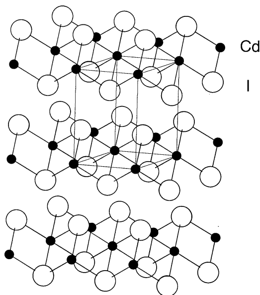
Fig. 4.24 Layers of cadmium and iodine in the cadmium iodide structure.
