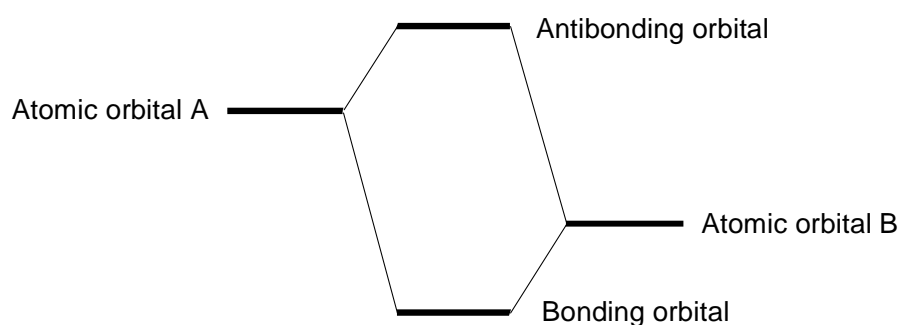
Fig. 2.15 Construction of molecular orbitals.
