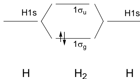
Fig. 2.18 The molecular orbitals of H_2 . The arrows indicate the electron spins.
