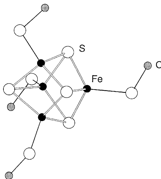
Fig. 6.25 Structure of [\text{Fe}_4\text{S}_4(\text{SR})_4]^{2-} .
