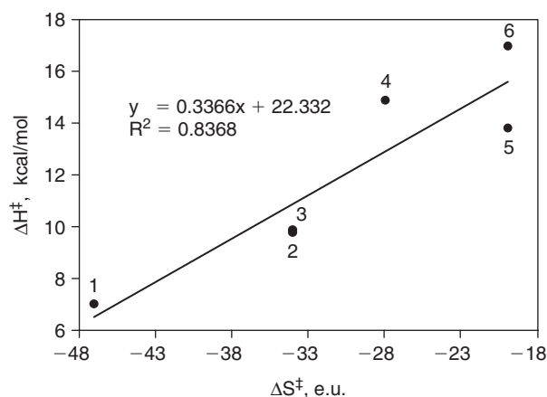
■ FIGURE 22.3 An isokinetic plot for oxidative addition of IrCl(CO)L_2 with CH_3I . The points 1 through 6 correspond to L = P\phi_3, PEt\phi_2, PEt_2\phi, P(p-C_6H_4CH_3)_3, P(p-C_6H_4F)_3, or P(p-C_6H_4Cl)_3 , respectively.
