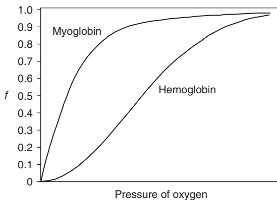
■ FIGURE 22.22 The qualitative relationship between the oxygen binding curves for hemoglobin and myoglobin.
