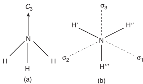
■ FIGURE 5.6 The pyramidal NH 3 molecule, which has C 3v symmetry. In (b), the C 3 axis is directed upward perpendicular to the plane of the paper at the nitrogen atom.
