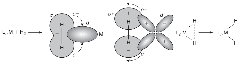
■ FIGURE 22.2 A possible mechanism for oxid of H_2 to a metal complex.
