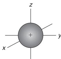
■ FIGURE 2.3 The three-dimensional surface representing the probability region of an s orbital.
