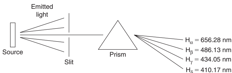
■ FIGURE 1.4 Separation of spectral lines due to refraction in a prism spectroscopy.
