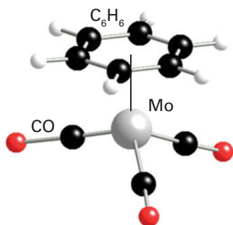
11 [\text{Mo}(\eta^6\text{-C}_6\text{H}_6)(\text{CO})_3]
