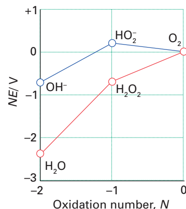
Fig. 5.7 The Frost diagram for oxygen in acidic solution (red line, \text{pH} = 0 ) and alkaline solution (blue line, \text{pH} = 14 ).
