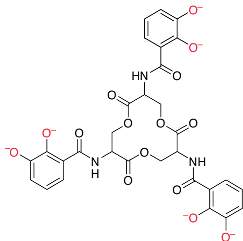
17 Enterobactin
