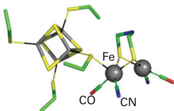
53 [FeFe]-hydrogenase
