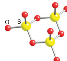
4 (\text{SO}_3)_n, C_{3v}
