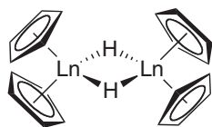
9 [(\text{Cp})_2\text{Ln}(\mu\text{-H})_2\text{Ln}(\text{Cp})_2]
