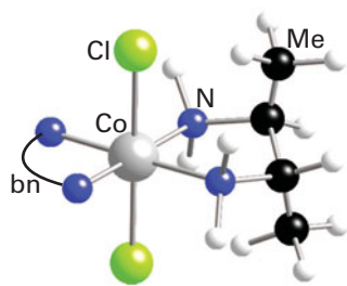
5 [\text{Co}(\text{Cl})_2(\text{bn})_2]^+
