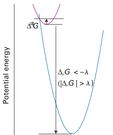
(c) Nuclear coordinates
