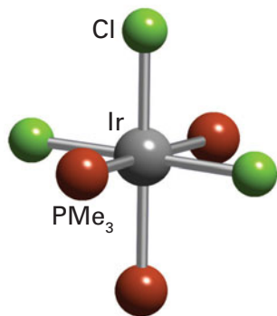
70 mer - [\text{IrCl}_3(\text{PMe}_3)_3]
