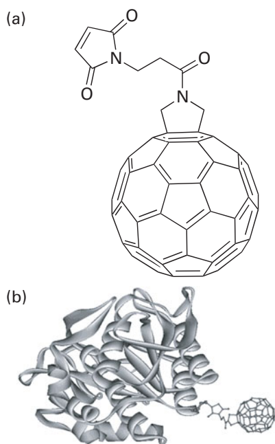
Figure 25.40 (a) Structure of N -(3-maleimidopropionyl)-3,4-fulleropyrrolidine. (b) The protein conjugated to N -(3-maleimidopropionyl)-3,4-fulleropyrrolidine (shown to scale). (P. Nednoor, et al. , Biocon. Chem. , 2004, 15 , 12.)
