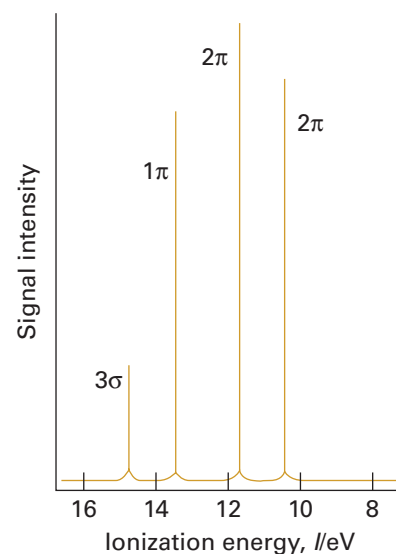
Figure 17.2 Photoelectron spectrum of ICl. The 2π levels give rise to two peaks because of spin-orbit interaction in the positive ion.
