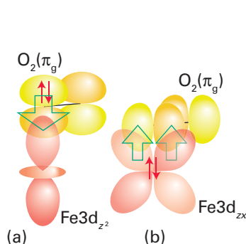
Figure 27.16 The orbitals used to form the Fe–O 2 adduct of myoglobin and haemoglobin. This model considers the O 2 ligand to be in a singlet state, in which the full 2\pi_g orbital donates an electron pair and the other 2\pi_g orbital acts as a \pi -electron pair acceptor.
