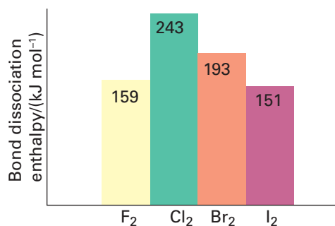
Figure 17.6 Bond dissociation enthalpies of the halogens in kilojoules per mole ( kJ\ mol^{-1} ).
