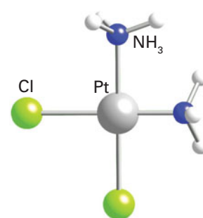
37 cis - [\text{PtCl}_2(\text{NH}_3)_2]
