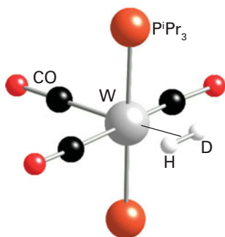
26 [\text{W}(\text{H}2)(\text{P}^i\text{Pr}_3)_2(\text{CO})_3] , ^i\text{Pr} = \text{CH}(\text{CH}_3)_2
