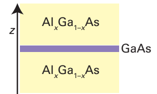
Figure 25.21 An (\text{Al}_x\text{Ga}_{1-x}\text{As})-(\text{GaAs})-(\text{Al}_x\text{Ga}_{1-x}\text{As}) quantum well; the thickness of the GaAs layer is on the nanoscale.
