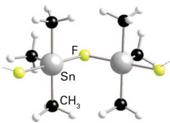
22 (\text{SnFMe}_3)_n , Me = CH 3
