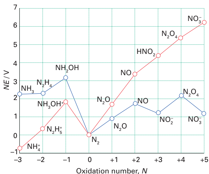
Fig. 5.6 The Frost diagram for nitrogen: the steeper the slope of a line, the higher the standard potential for the couple. The red line refers to standard (acid) conditions ( \text{pH} = 0 ), the blue line refers to \text{pH} = 14 . Note that because \text{HNO}_3 is a strong acid, even at \text{pH} = 0 it is present as its conjugate base \text{NO}_3^- .
