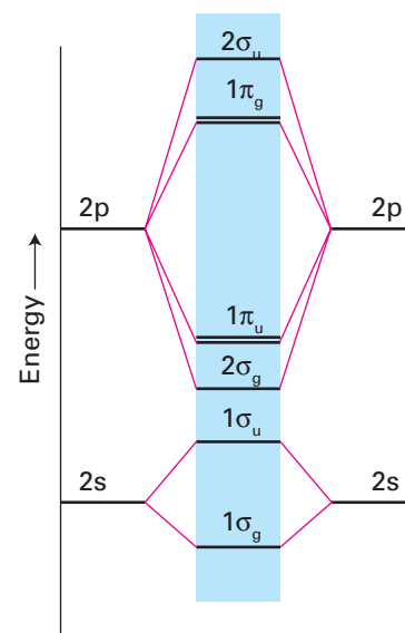
Fig. 2.12 The molecular orbital energy level diagram for the later Period 2 homonuclear diatomic molecules. This diagram should be used for O_2 and F_2 .
