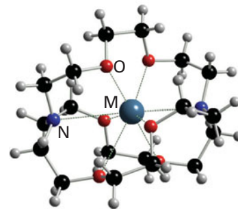
4 2.2.2-crypt complex
