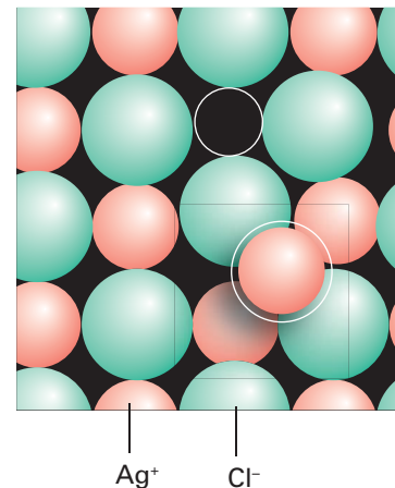
Fig. 3.54 A Frenkel defect forms when an ion moves to an interstitial site.
