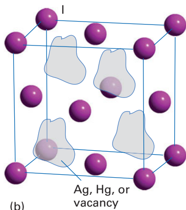
Figure 24.5 (a) Low-temperature ordered structure of \text{Ag}_2\text{HgI}_4 . (b) High-temperature disordered structure showing the cation disorder. \text{Ag}_2\text{HgI}_4 is an \text{Ag}^+ ion conductor in the high temperature form.
