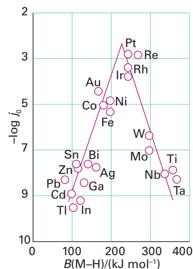
Figure 26.28 The rate of H_2 evolution expressed as the logarithm of the exchange current density plotted against M–H bond energy.
