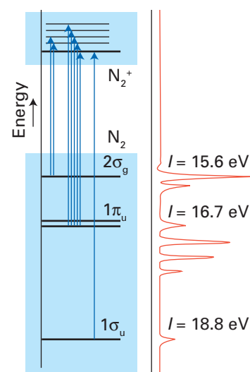
Fig. 2.11 The UV photoelectron spectrum of N_2 . The fine structure in the spectrum arises from excitation of vibrations in the cation formed by photoejection of an electron.
