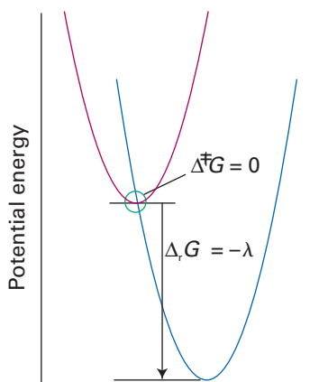
(b) Nuclear coordinates
