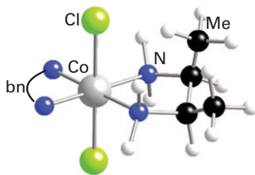
6 [\text{Co}(\text{Cl})_2(\text{bn})_2]^+
