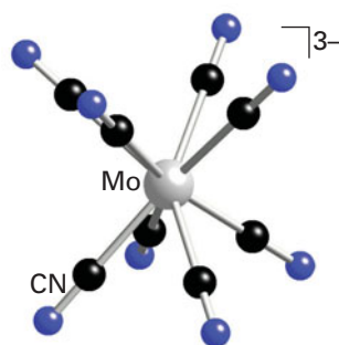
28 [\text{Mo}(\text{CN})_8]^{3-} ( D_4 )
