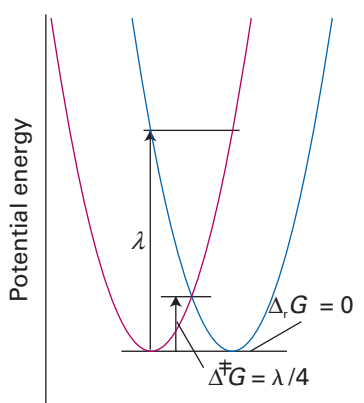
(a) Nuclear coordinates
