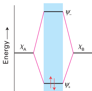
Fig. 2.10 The molecular orbital energy level diagram for H_2 and analogous molecules.
