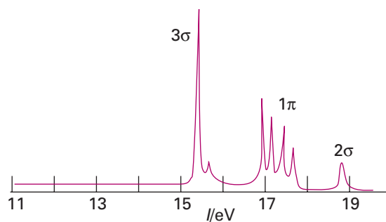
Fig. 2.39 The UV photoelectron spectrum of \text{CO} obtained using 21 eV radiation.
