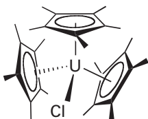
13 \text{U}(\text{Cp}^*)_3\text{Cl}
