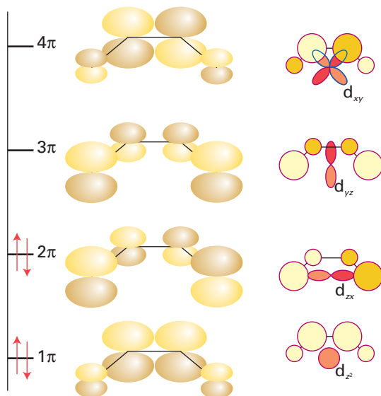
Figure 22.6 The molecular orbitals of the \pi system in butadiene; also shown are metal d orbitals of appropriate symmetry to form bonding interactions.
