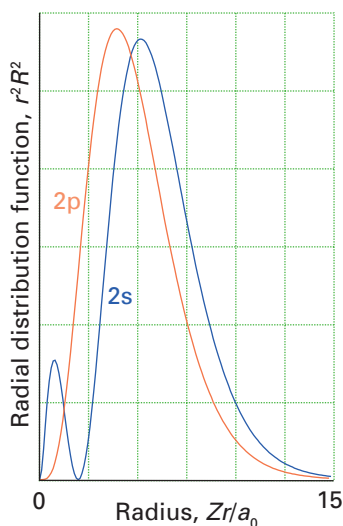
Figure 1.12 The radial distribution functions of hydrogenic orbitals. Although the 2p orbital is on average closer to the nucleus (note where its maximum lies), the 2s orbital has a high probability of being close to the nucleus on account of the inner maximum.
