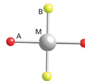
40 trans - [\text{MA}_2\text{B}_2]
