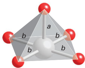
53 Square pyramid ( C_{4v} )
