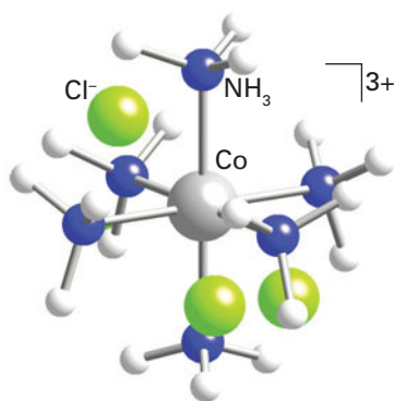
2 [Co(NH 3 ) 6 ]Cl 3
