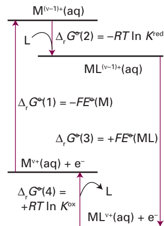
Fig. 5.4 Thermodynamic cycle showing how the standard potential of the couple M^{v+}/M is altered by the presence of a ligand L.
