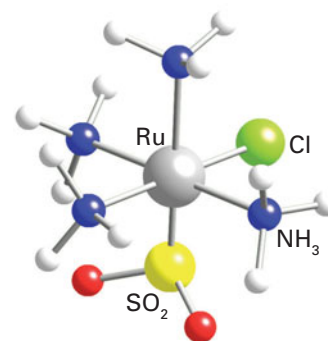
23 [\text{RuCl}(\text{NH}_3)_4(\text{SO}_2)]^+
