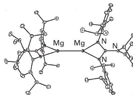
13 LMgMgL , L = [Ar(NC)(N^iPr_2)NAr]^- \cdot iPr = (CH_3)_2CH
