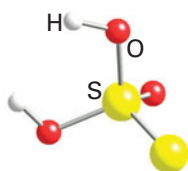
27 Thiosulfuric acid, \text{H}_2\text{S}_2\text{O}_3
