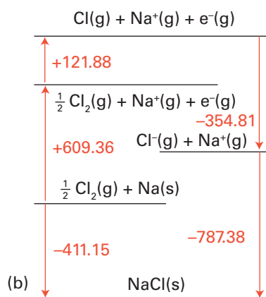
Figure 17.1 Thermochemical cycles for (a) sodium fluoride and (b) sodium chloride. All values are in kilojoules per mole (kJ mol -1 ).
