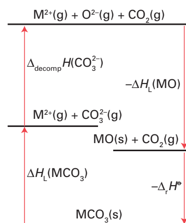
Fig. 3.49 A thermodynamic cycle showing the enthalpy changes involved in the decomposition of a solid carbonate \text{MCO}_3 .
