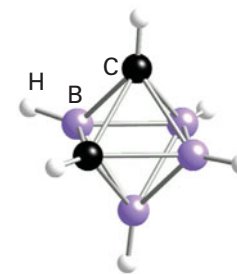
10 closo -1,2- \text{B}_4\text{C}_2\text{H}_6
