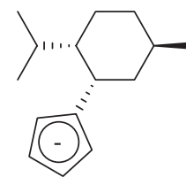
47 neo-Menthylcyclopentadienyl
