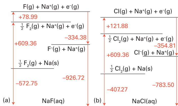
Figure 17.10 Thermochemical cycles for the enthalpy of formation of (a) aqueous sodium fluoride and (b) aqueous sodium chloride. The hydration is much more exothermic for \text{F}^- than for \text{Cl}^- . All values are in kilojoules per mole ( \text{kJ mol}^{-1} ).
