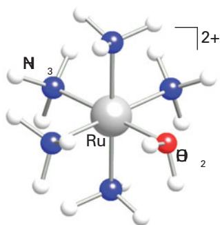
1 [Ru(OH_2)(NH_3)_5]^{2+}
