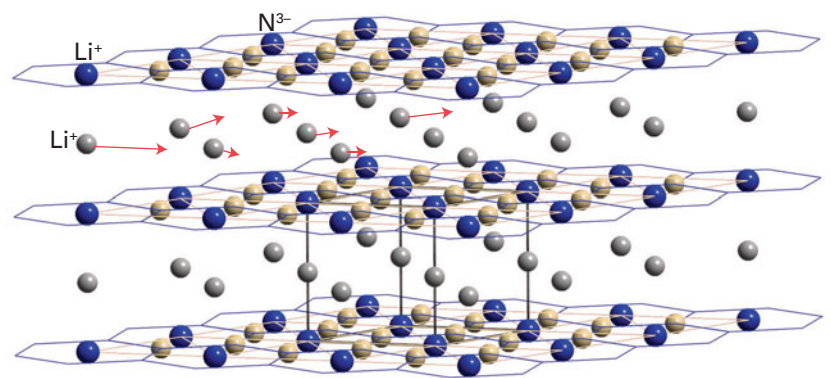
Figure 24.8 The \text{Li}_3\text{N} structure showing possible pathways for \text{Li}^+ ion diffusion between the \text{Li}_2\text{N} planes.
