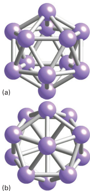
Figure 13.1 A view of the B_{12} icosahedron in \alpha -rhombohedral boron (a) along and (b) perpendicular to the threefold axis of the crystal. The individual icosahedra are linked by 3c, 2e bonds.
