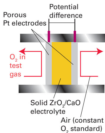
Figure 24.9 An oxygen sensor based on the solid electrolyte Zr_{1-x}Ca_xO_{2-x} .
