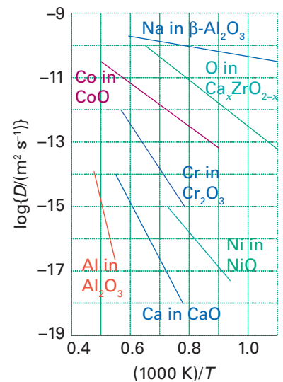
Figure 24.4 The diffusion coefficients (on a logarithmic scale) as a function of inverse temperature for the mobile ion in selected solids.
