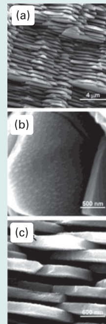
Figure B25.4 SEM images of the nacreous fracture shell section taken at increasing magnification. The brick-and-mortar architecture is shown in (a) and (c). Nanoscale asperities on the aragonite platelet surface are readily observed in (b). (X. Li, et al. , Nano Lett. , 2004, 4, 613.)
