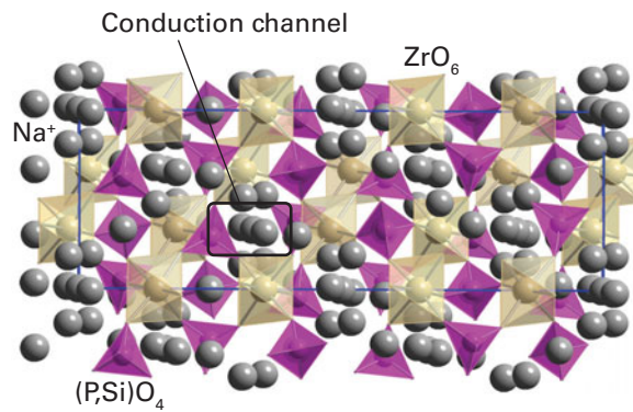
Figure 24.7 The \text{Na}_{1+x}\text{Zr}_2\text{P}_{3-x}\text{Si}_x\text{O}_{12} (NASICON) structure shown as linked (\text{P,Si})\text{O}_4 tetrahedra and \text{ZrO}_6 .
