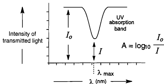
Figure 2.2 Definition of Absorbance (A)
