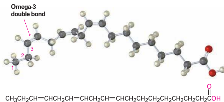
Linolenic acid, an omega-3 polyunsaturated fatty acid
