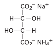
Sodium ammonium tartrate
