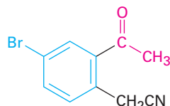
9. (2-Acetyl-4-bromophenyl)acetonitrile
