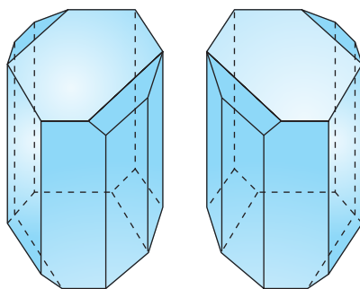
FIGURE 5-6 Drawings of sodium ammonium tartrate crystals taken from Pasteur's original sketches. One of the crystals is dextrorotatory in solution, and the other is levorotatory.
