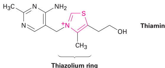
Thiazolium ring
