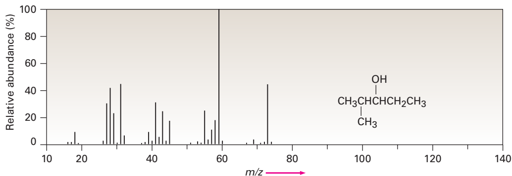
FIGURE 12-14 Mass spectrum of 2-methyl-3-pentanol, Worked Example 12-2.
