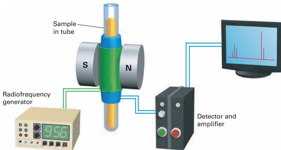
FIGURE 13-4 Schematic operation of a basic NMR spectrometer. A thin glass tube containing the sample solution is placed between the poles of a strong magnet and irradiated with rf energy.
