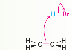
Ethylene
