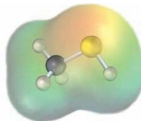
Methanethiol
