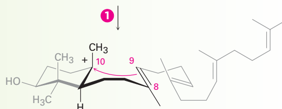
(3S)-2,3-Oxidosqualene
