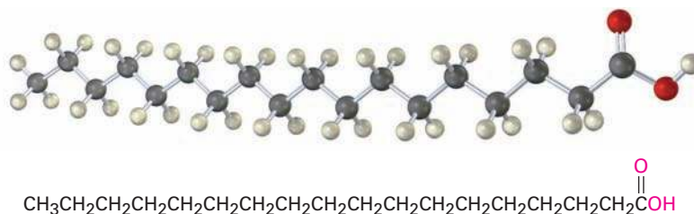
Stearic acid
