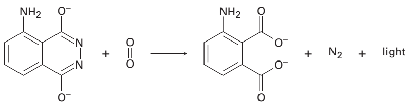
Luminol dianion
