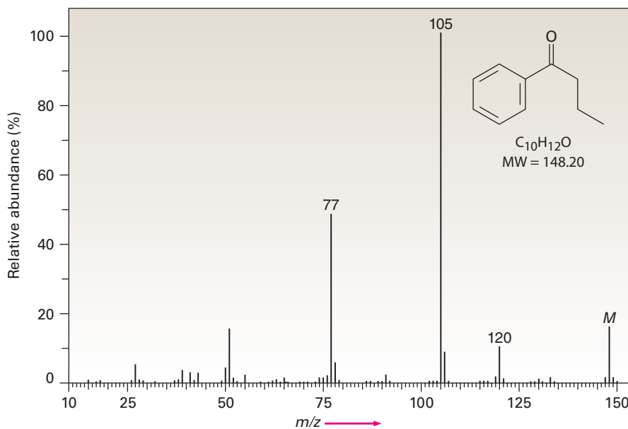
FIGURE 12-13 Mass spectrum of butyrophenone.
