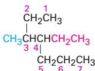
4-Ethyl-3-methylheptane
