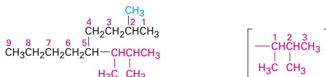
5-(1,2-Dimethylpropyl)-2-methylnonane
