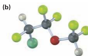
Enflurane (an anesthetic)
