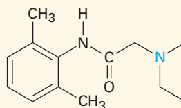
Lidocaine (Xylocaine)
