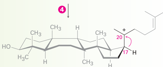
Protosteryl cation
