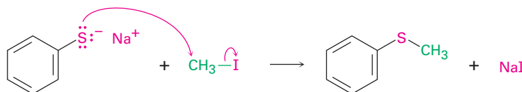
Sodium benzenethiolate
