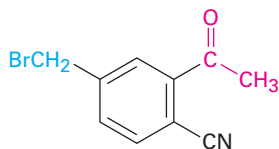
8. 2-Acetyl-(4-bromomethyl)benzonitrile
