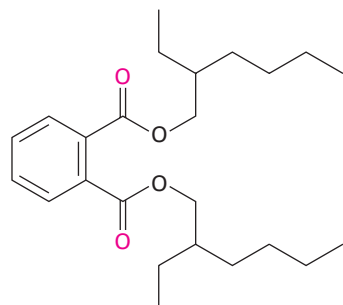
Di(2-ethylhexyl) phthalate (or dioctyl phthalate), a plasticizer
