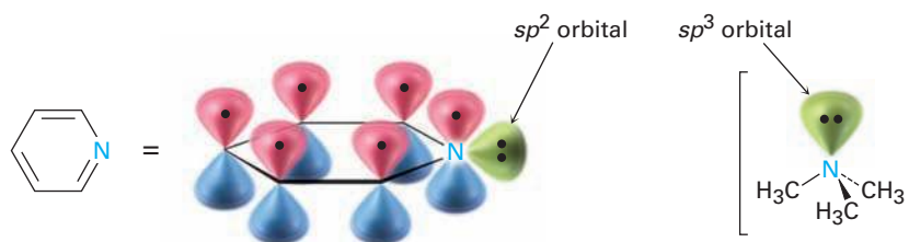
Pyridine
