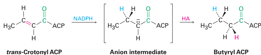
FIGURE 8-7 Reduction of the carbon–carbon double bond in trans -crotonyl ACP, a step in the biosynthesis of fatty acids. One hydrogen is delivered from NADPH as a hydride ion, \text{H}^- ; the other hydrogen is delivered by protonation of the anion intermediate with an acid, HA.
